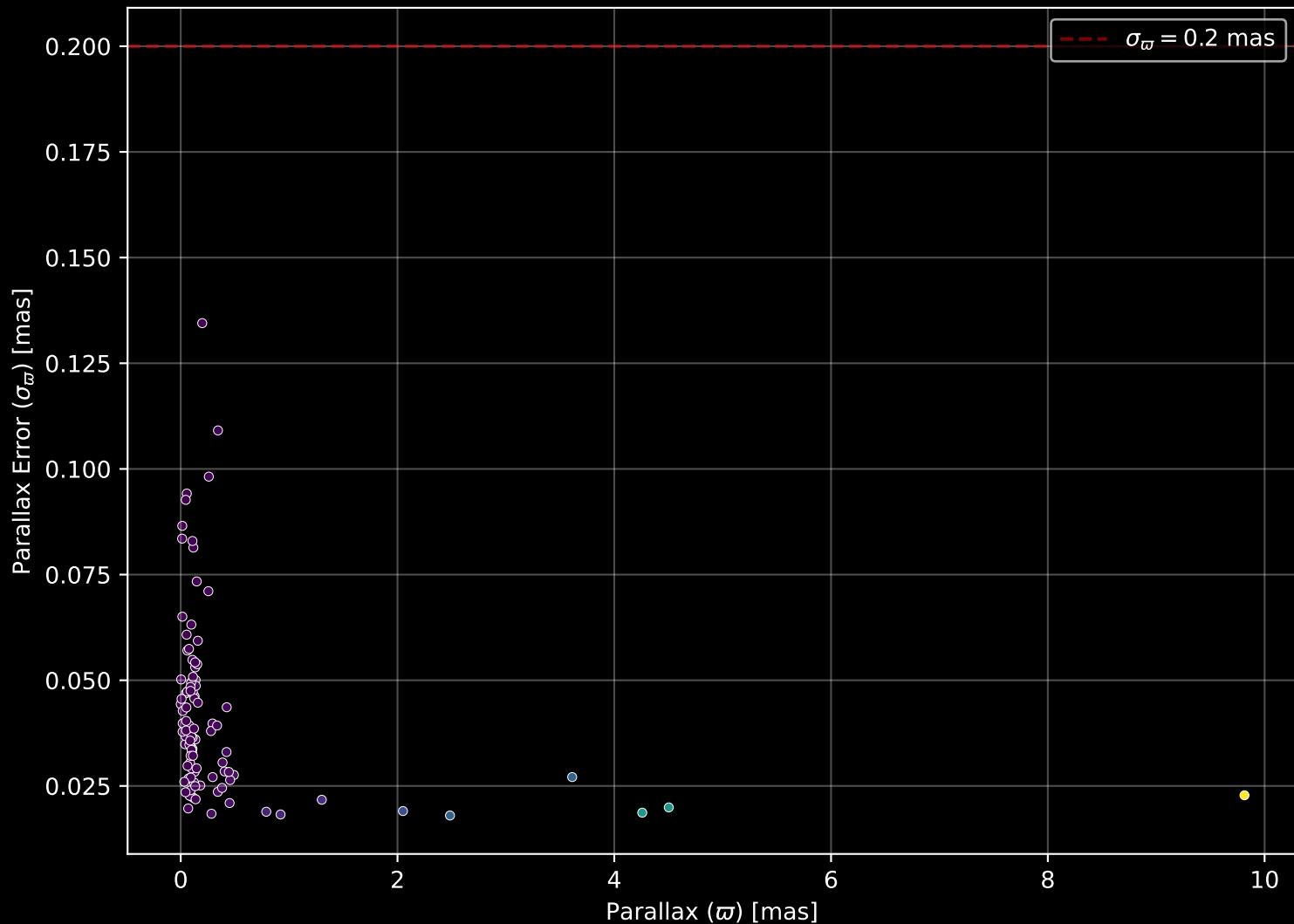
APOGEE DR17 Field: [INTCL_N6316_MGA] Parallax Quality (n= 102)
