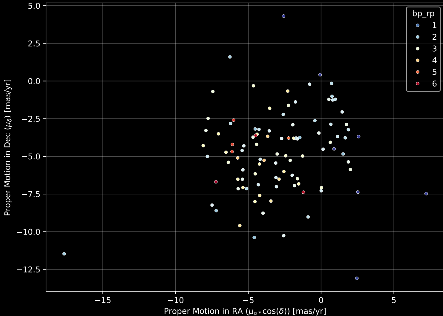
APOGEE DR17 Field: [INTCL_N6316_MGA] Proper Motion Diagram (n= 102)
