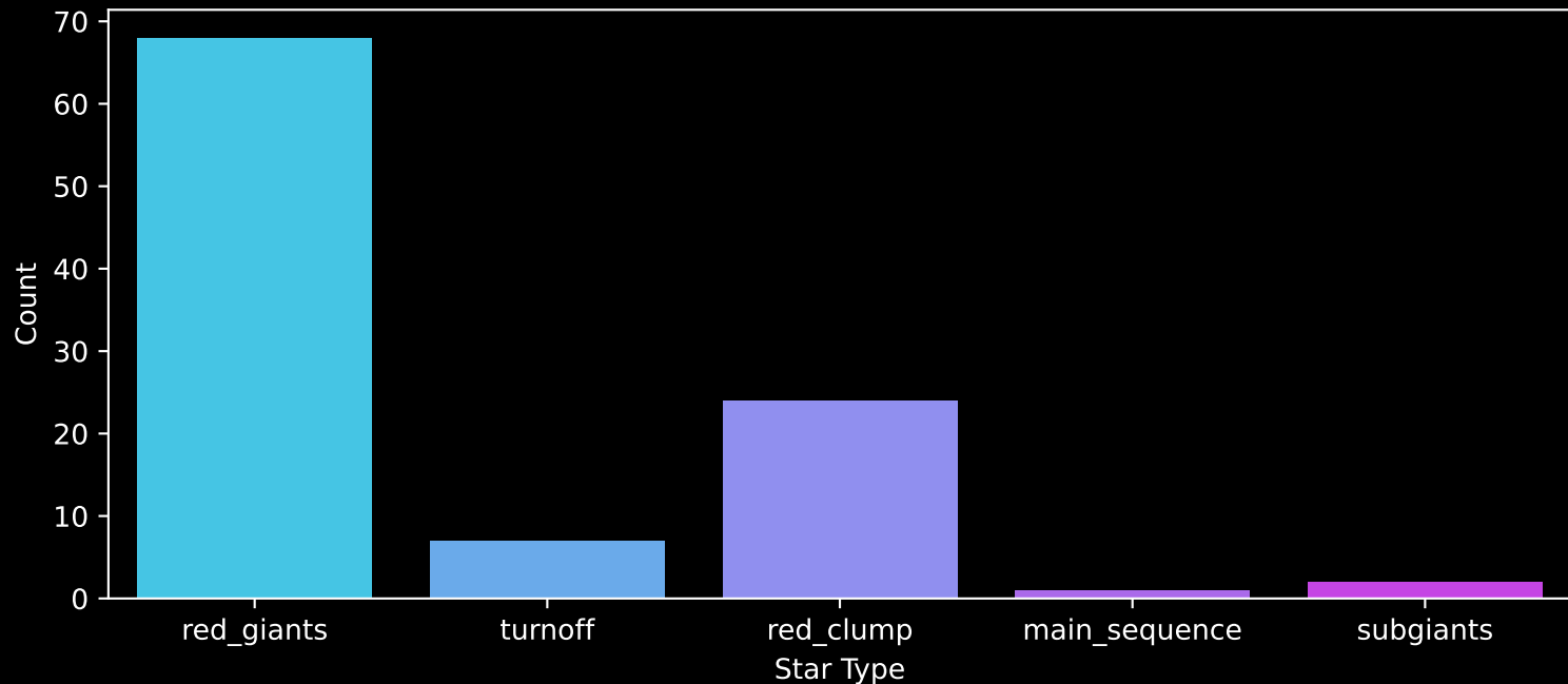
APOGEE DR17 Field: [INTCL_N6316_MGA] Count plot of Star Type
