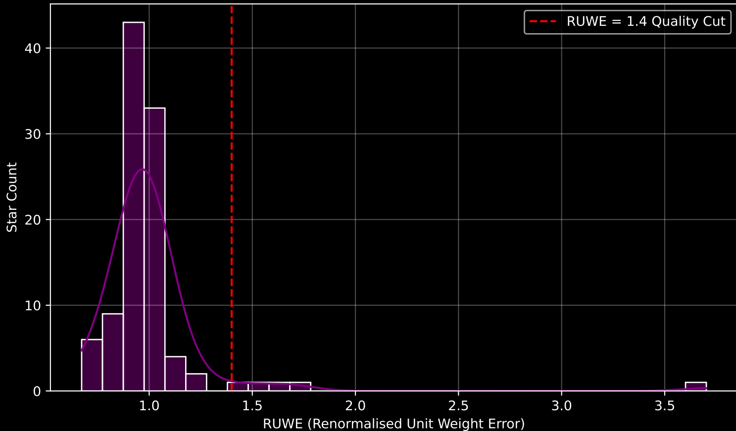
GAPOGEE DR17 Field [INTCL_N6316_MGA] RUWE Distribution (n= 102)
