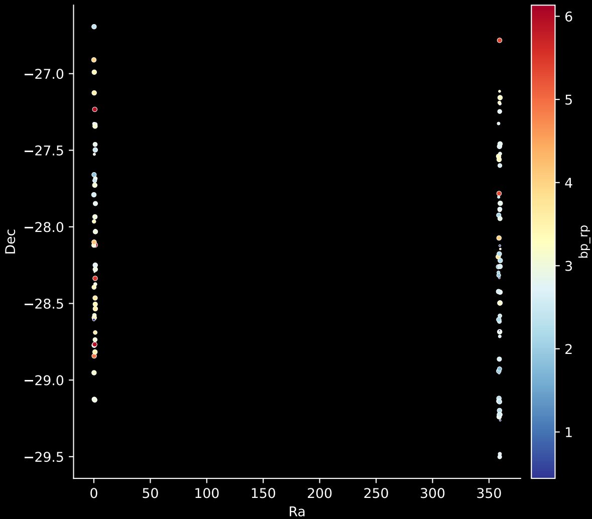
APOGEE DR17 Field: [INTCL_N6316_MGA] Stars: 102
