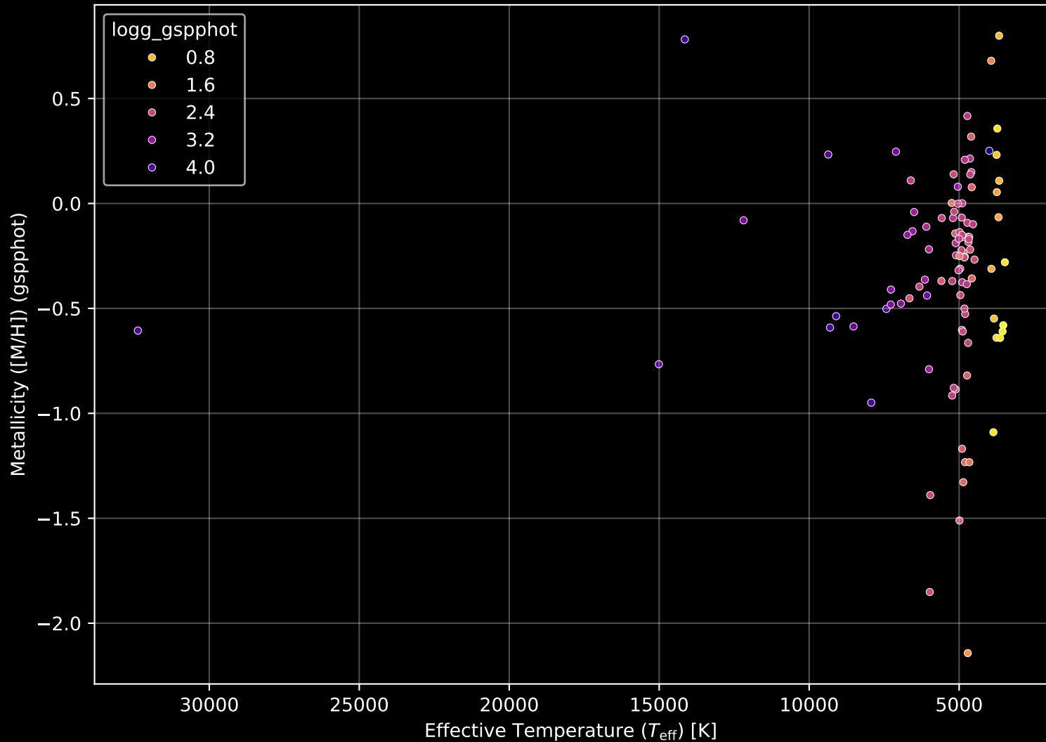
APOGEE DR17 Field: [INTCL_N6316_MGA] Stellar Population Parameters (n= 102)
