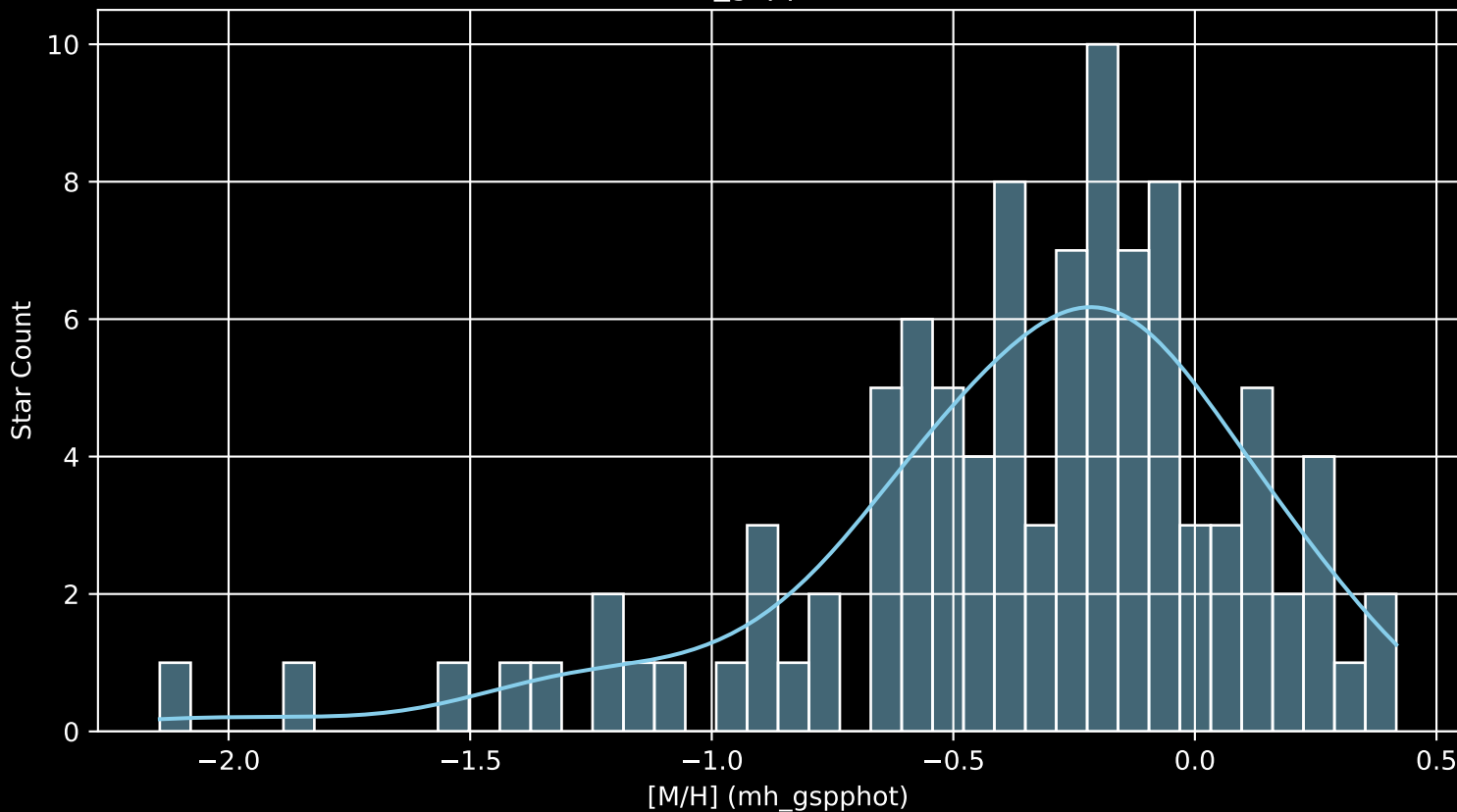
APOGEE DR17 Field: [INTCL_N6316_MGA [M/H] (mh_gspphot) (n= 99)
